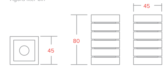
Agora litter-bin
